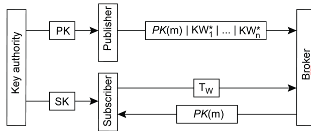
Figure 5.35: The principle of privacy-preserving publish-subscribe.
