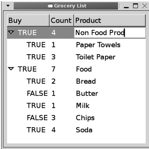
Figure 8-8. An editable cell
