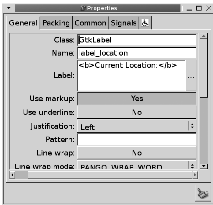
Figure 10-10. GtkLabel widget properties
