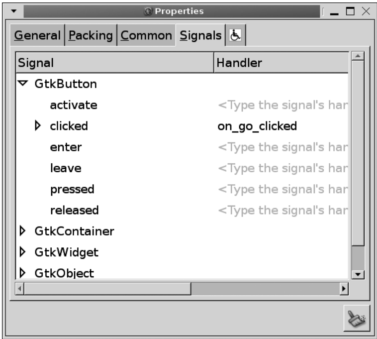
Figure 10-12. A widget signal editor
