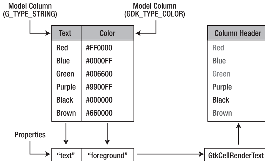
Figure 8-3. Applying Cell Renderer Properties
