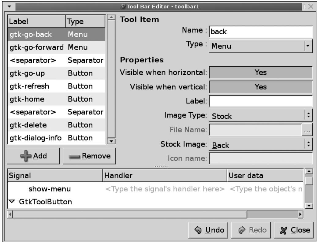
Figure 10-6. The toolbar editor
