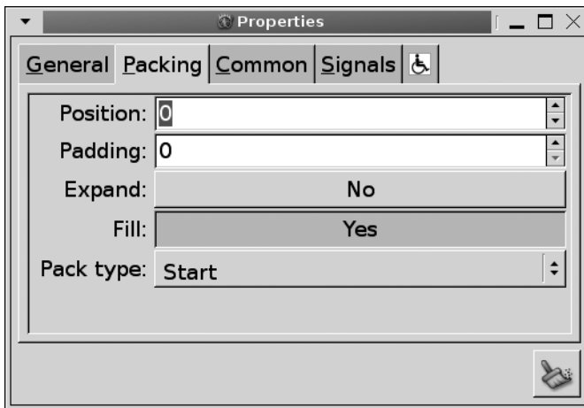
Figure 10-7. Widget packing properties
