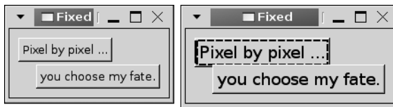
Figure 3-6. Problems caused by different font sizes in a GtkFixed container
