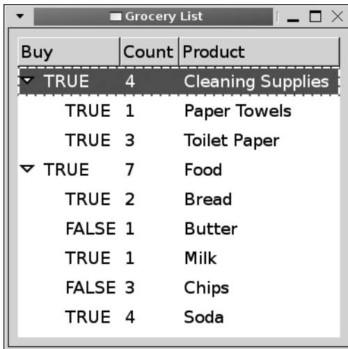
Figure 8-5. A tree view widget using a GtkTreeStore tree model
