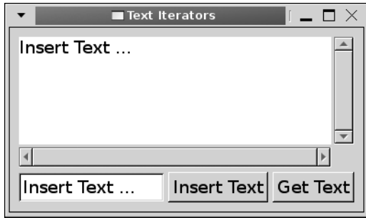
Figure 7-4. Screenshot of an application using a GtkTextView widget
