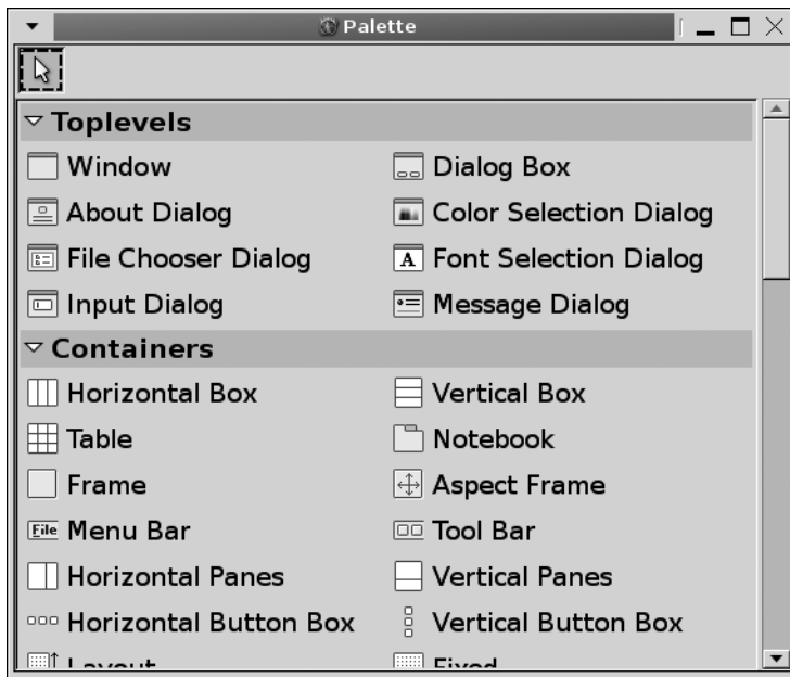
Figure 10-2. The Glade widget palette
