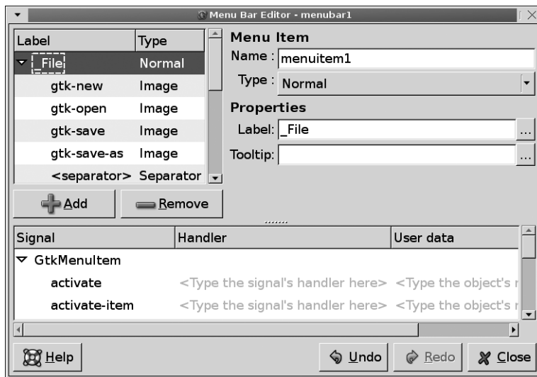
Figure 10-13. The Menu Bar Editor
