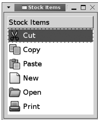
Figure 8-11. Pixbuf renderers
