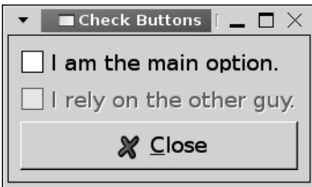
Figure 4-3. Check buttons
