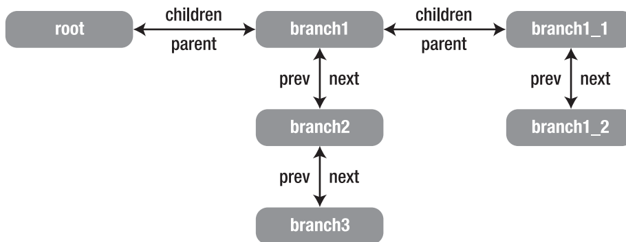
Figure 6-1. GNode relationships
