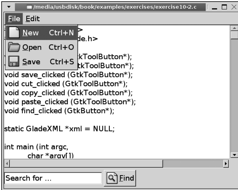
Figure F-2. The text editor application with a menu bar in Glade
