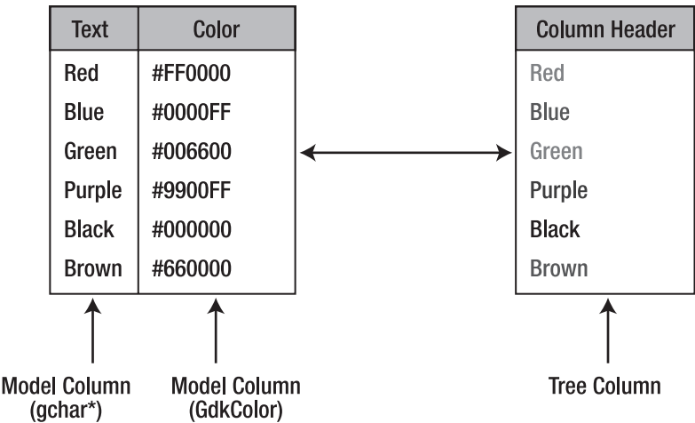
Figure 8-2. The relationship between model and tree columns
