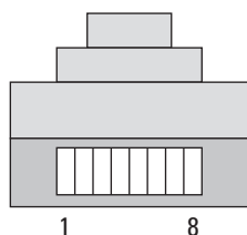
Figure 5-2: Front view of an RJ-45 connector showing the pin numbers
